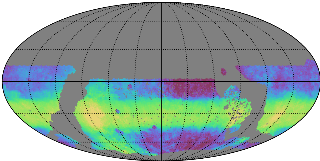
too_elab_r8_d3_giz_v3.4_10yrs WFD y band: Median HA
