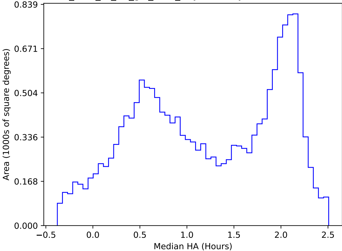
too_elab_r8_d3_giz_v3.4_10yrs WFD y band: Median HA
