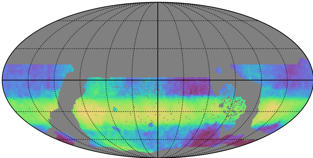
too_elab_r8_d3_giz_v3.4_10yrs WFD r band: Median HA
