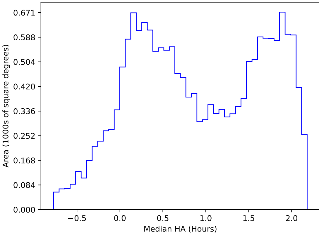
too_elab_r8_d3_giz_v3.4_10yrs WFD r band: Median HA
