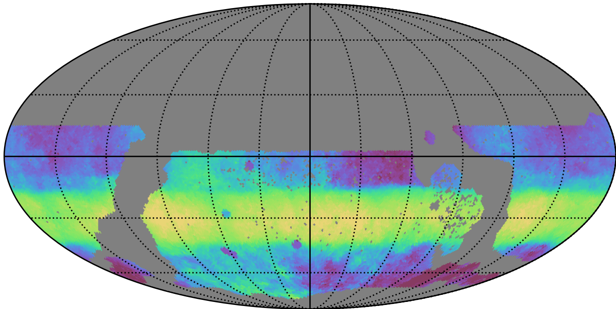
too_elab_r8_d3_giz_v3.4_10yrs WFD i band: Median HA
