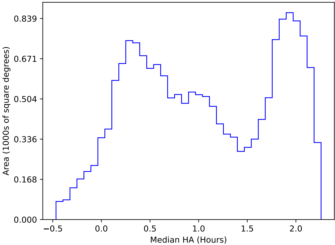
too_elab_r8_d3_giz_v3.4_10yrs WFD i band: Median HA
