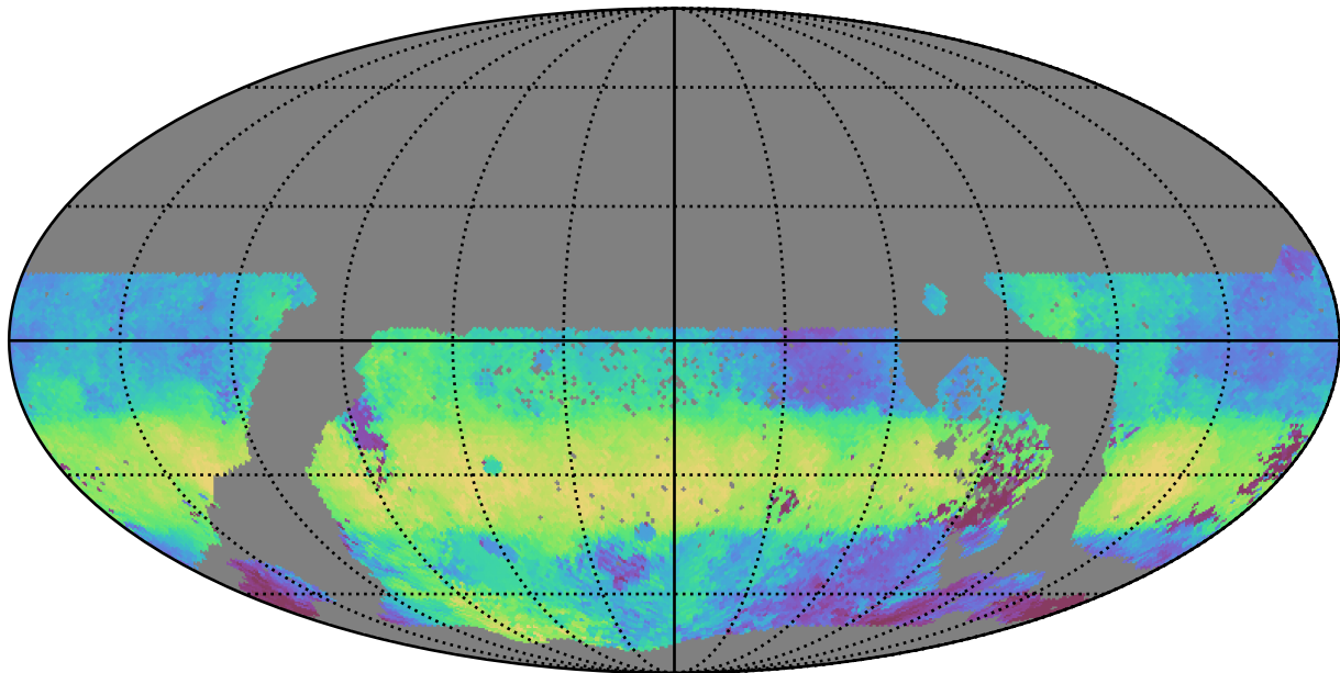
too_elab_r8_d3_giz_v3.4_10yrs WFD g band: Median HA
