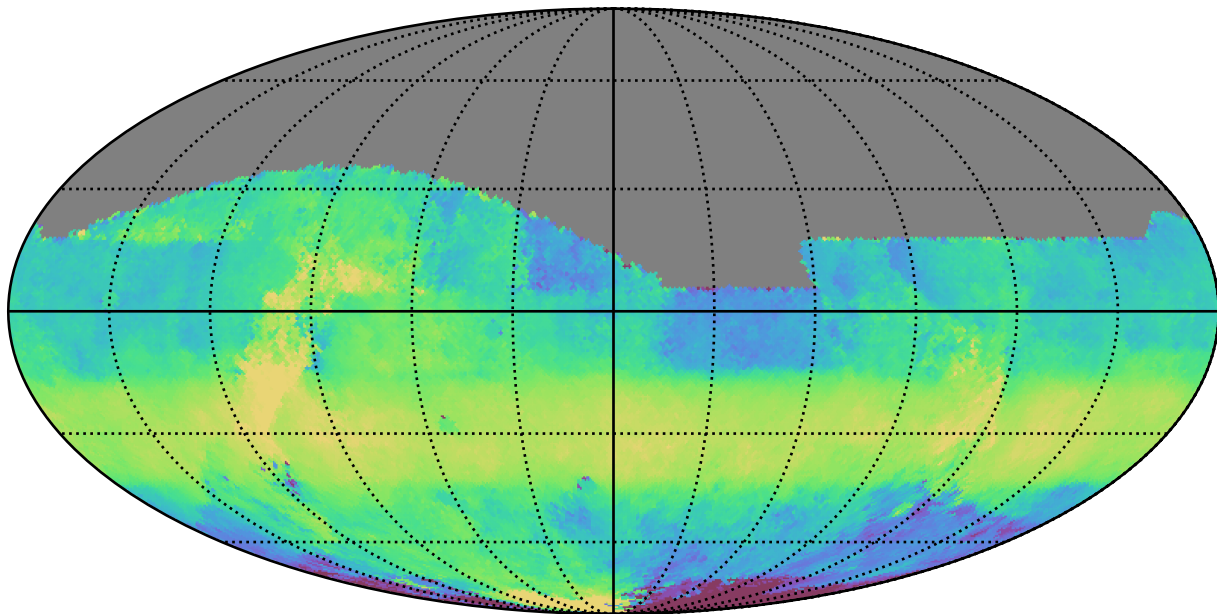
too_elab_r8_d3_giz_v3.4_10yrs All sky z band: Median HA
