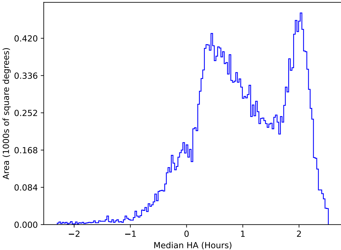
too_elab_r8_d3_giz_v3.4_10yrs All sky z band: Median HA
