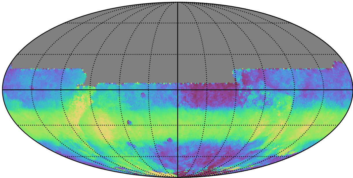
too_elab_r8_d3_giz_v3.4_10yrs All sky y band: Median HA
