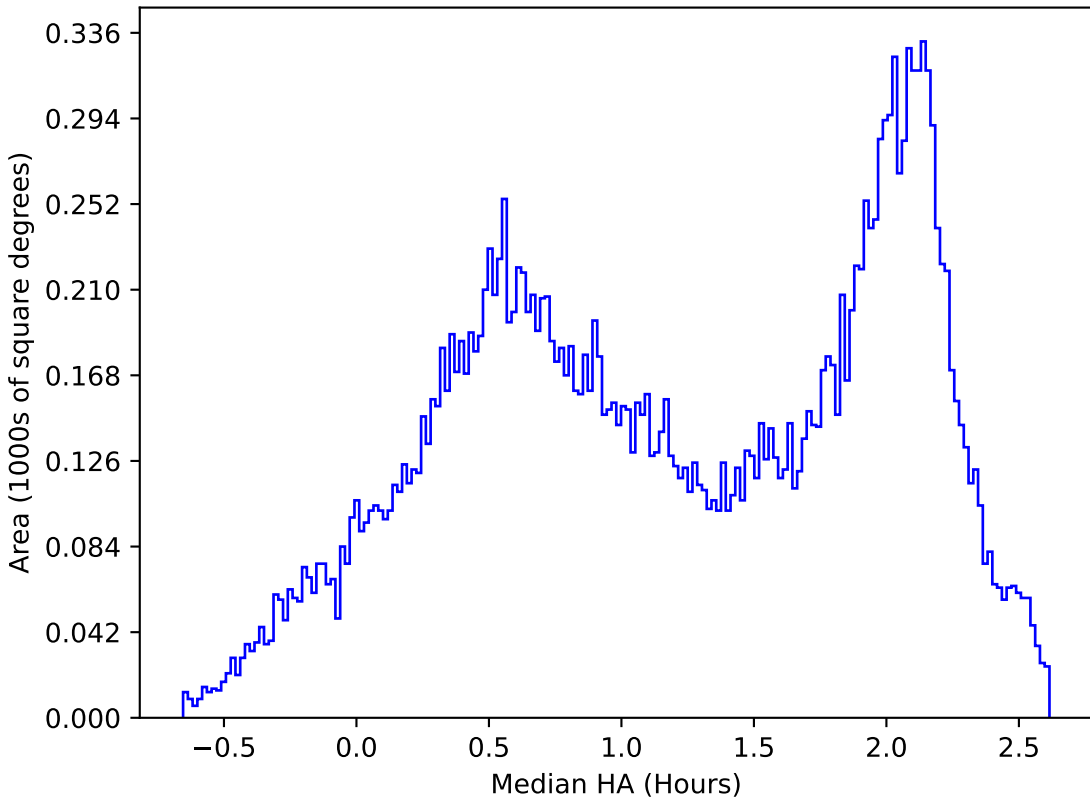
too_elab_r8_d3_giz_v3.4_10yrs All sky y band: Median HA
