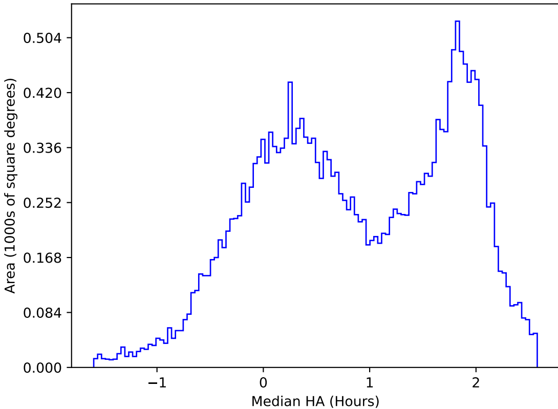
too_elab_r8_d3_giz_v3.4_10yrs All sky u band: Median HA
