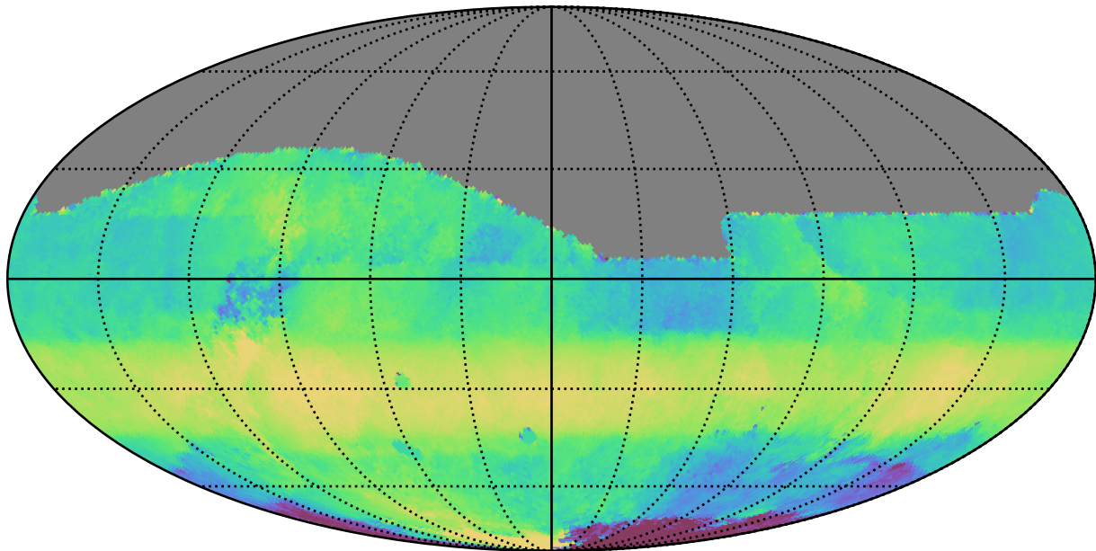
too_elab_r8_d3_giz_v3.4_10yrs All sky r band: Median HA
