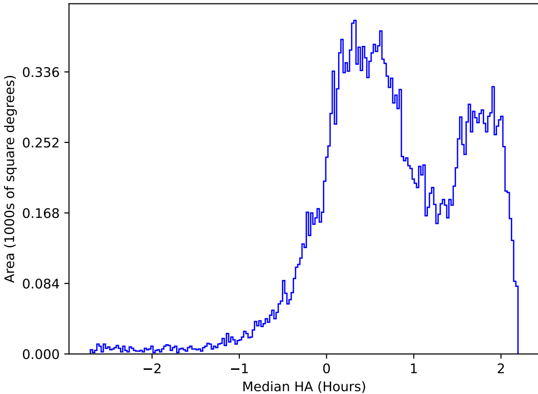
too_elab_r8_d3_giz_v3.4_10yrs All sky r band: Median HA
