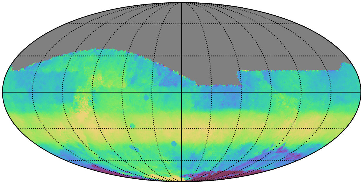
too_elab_r8_d3_giz_v3.4_10yrs All sky i band: Median HA
