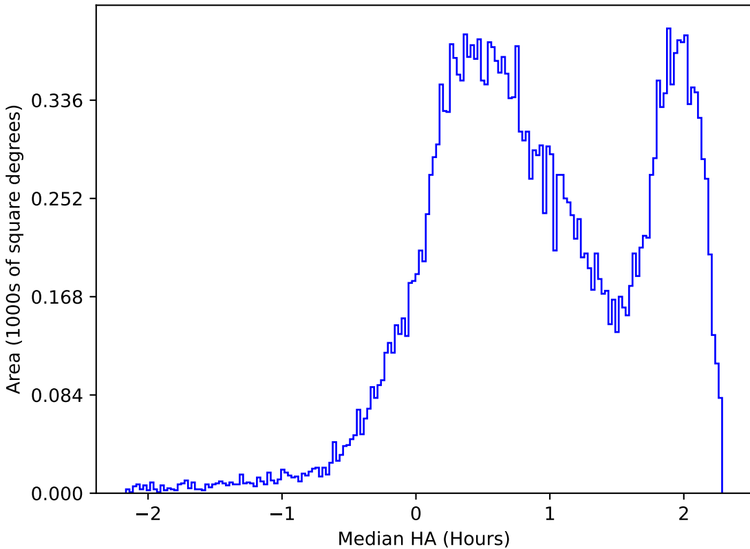
too_elab_r8_d3_giz_v3.4_10yrs All sky i band: Median HA
