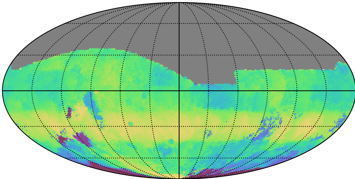
too_elab_r8_d3_giz_v3.4_10yrs All sky g band: Median HA
