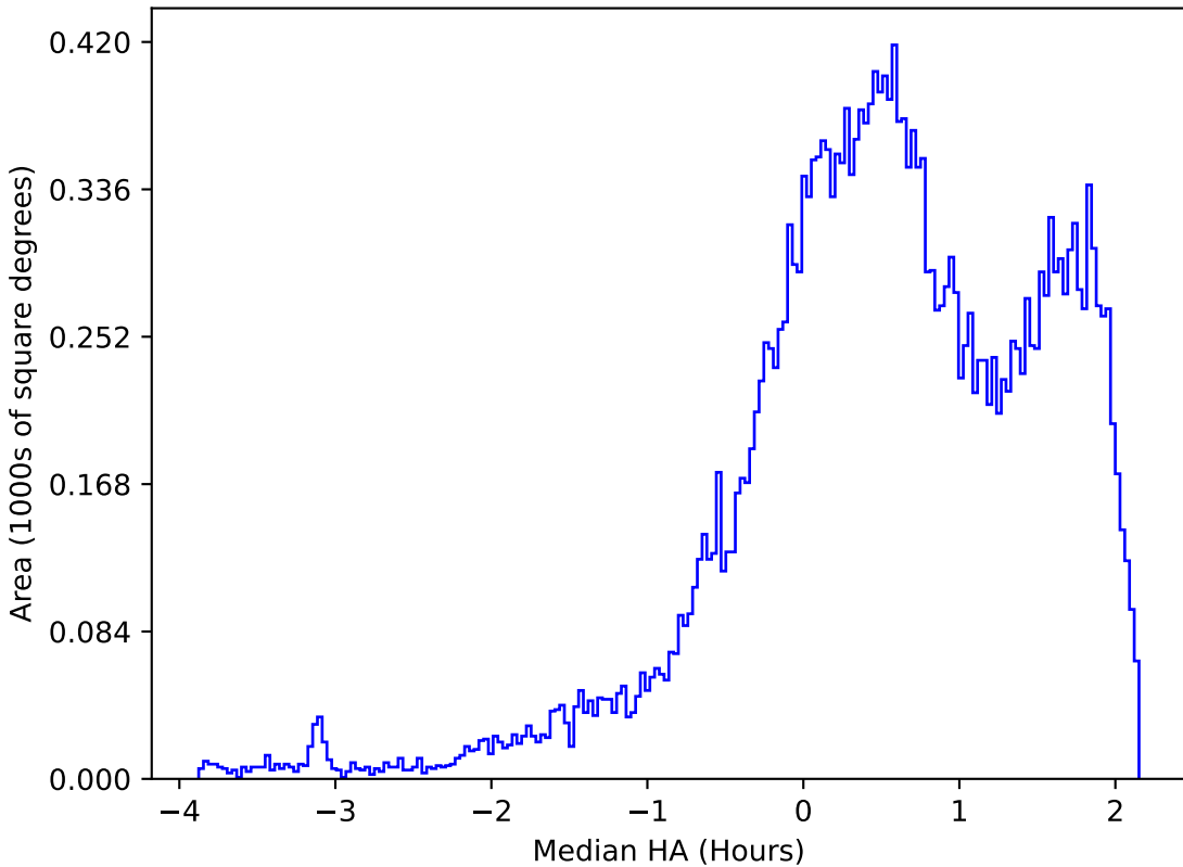
too_elab_r8_d3_giz_v3.4_10yrs All sky g band: Median HA
