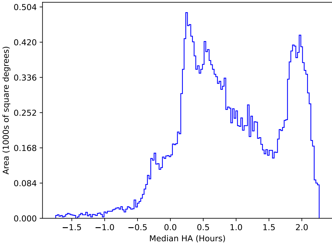
too_elab_r8_d3_giz_v3.4_10yrs All sky all bands: Median HA
