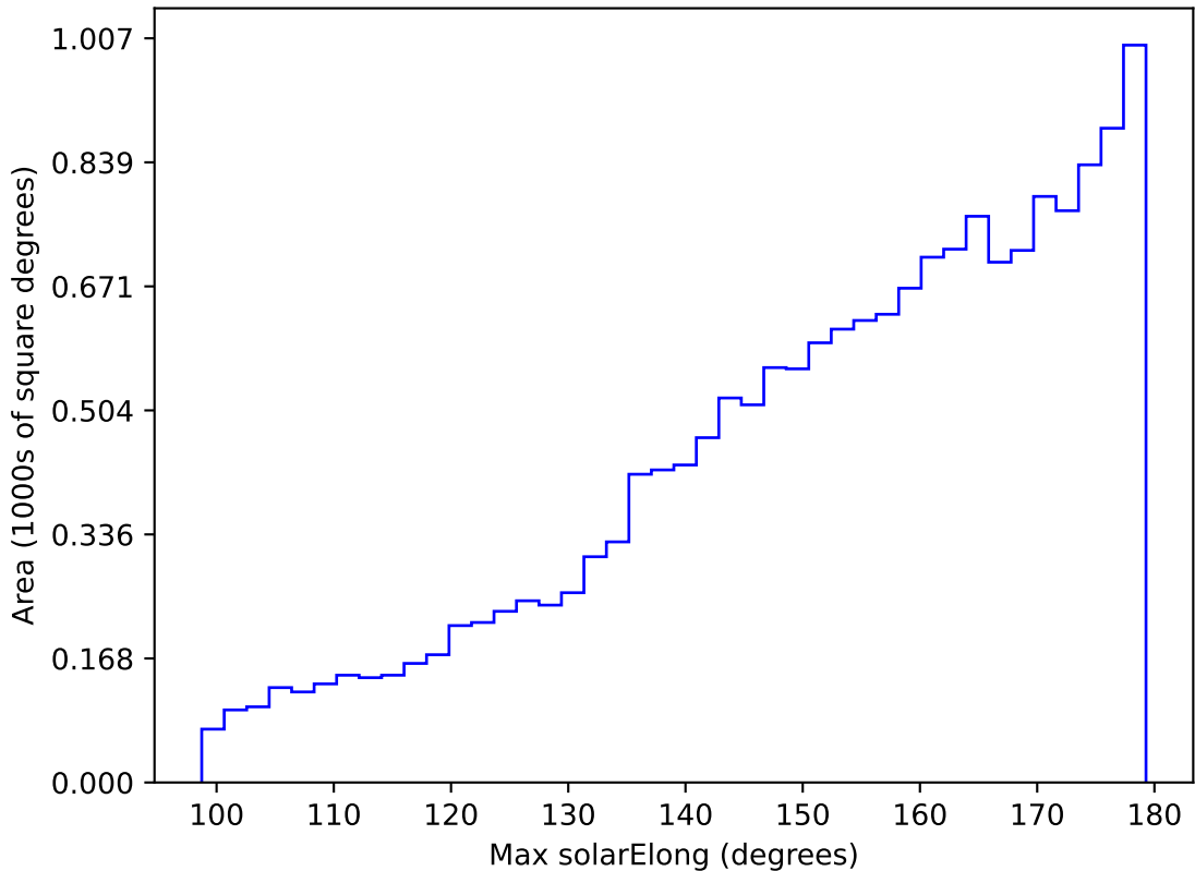
too_elab_r8_d3_giz_v3.4_10yrs WFD y band: Max solarElong
