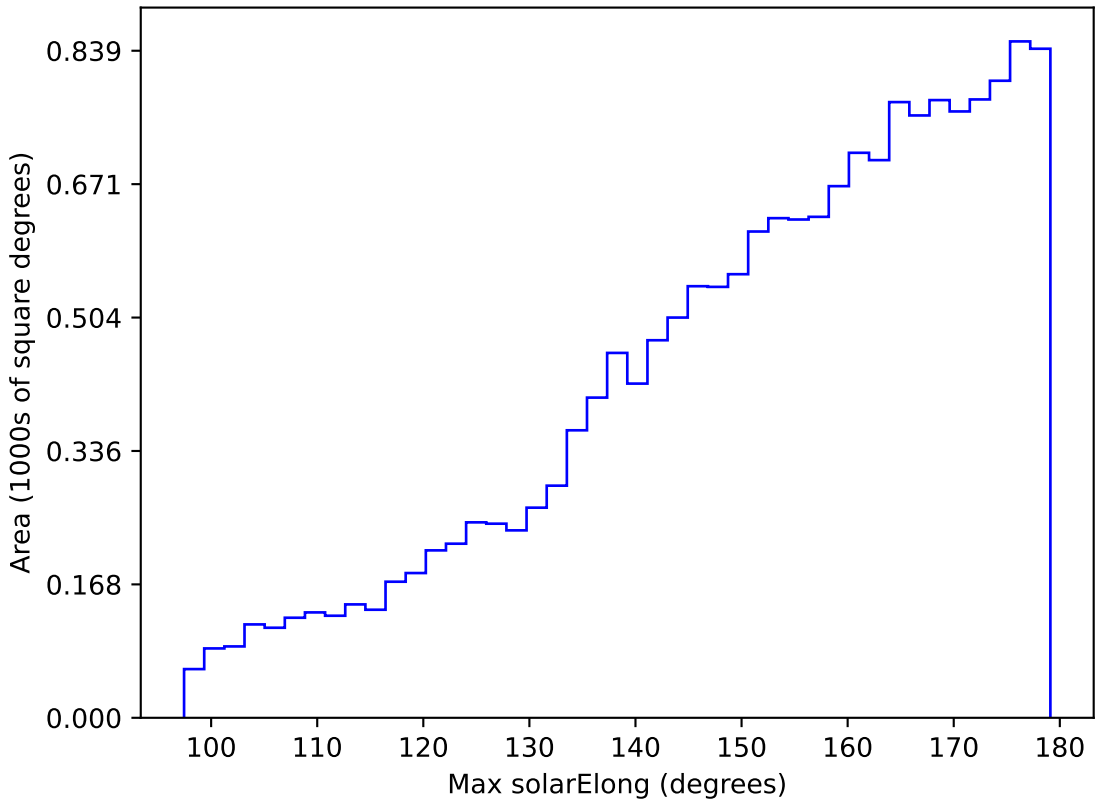
too_elab_r8_d3_giz_v3.4_10yrs WFD u band: Max solarElong
