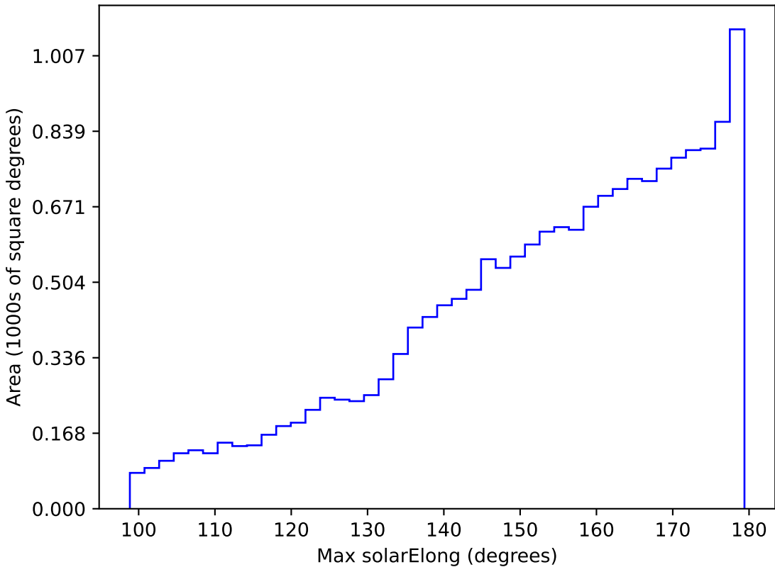
too_elab_r8_d3_giz_v3.4_10yrs WFD r band: Max solarElong
