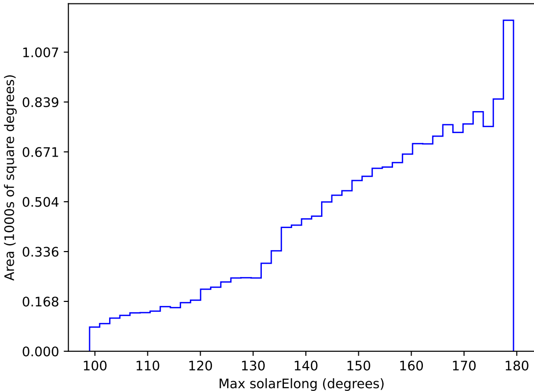
too_elab_r8_d3_giz_v3.4_10yrs WFD i band: Max solarElong
