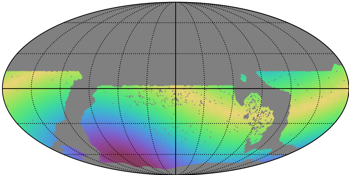
too_elab_r8_d3_giz_v3.4_10yrs WFD g band: Max solarElong
