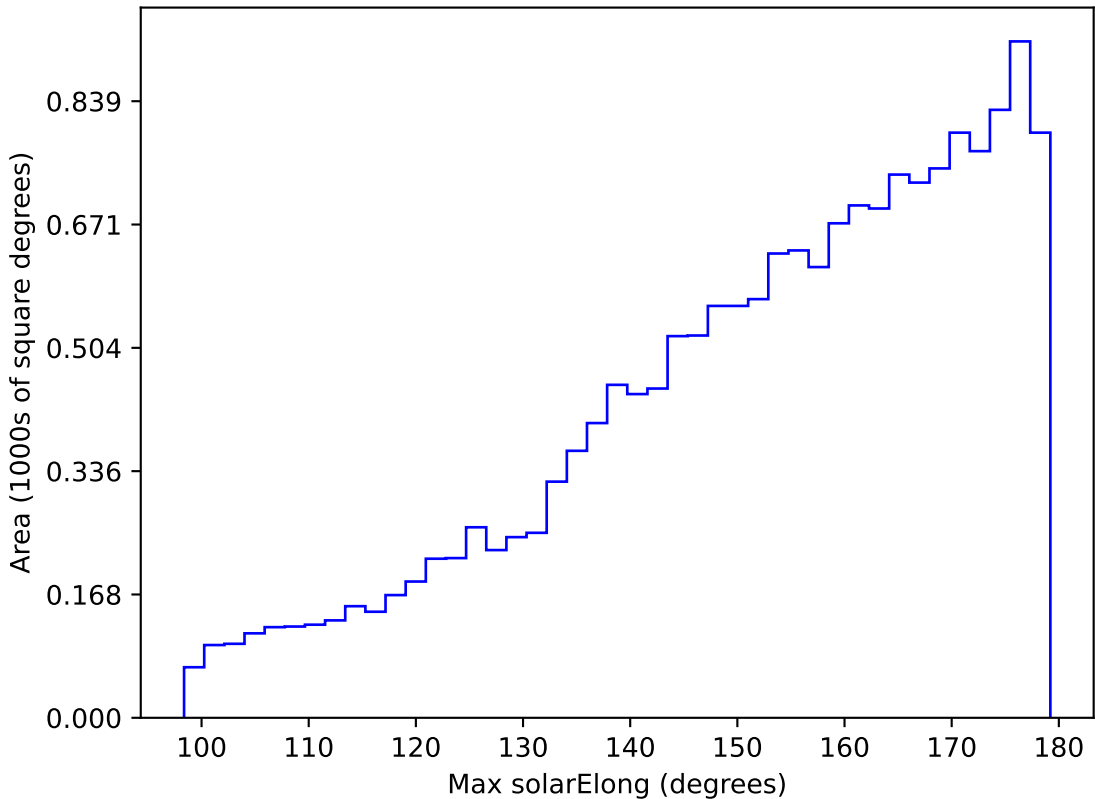
too_elab_r8_d3_giz_v3.4_10yrs WFD g band: Max solarElong
