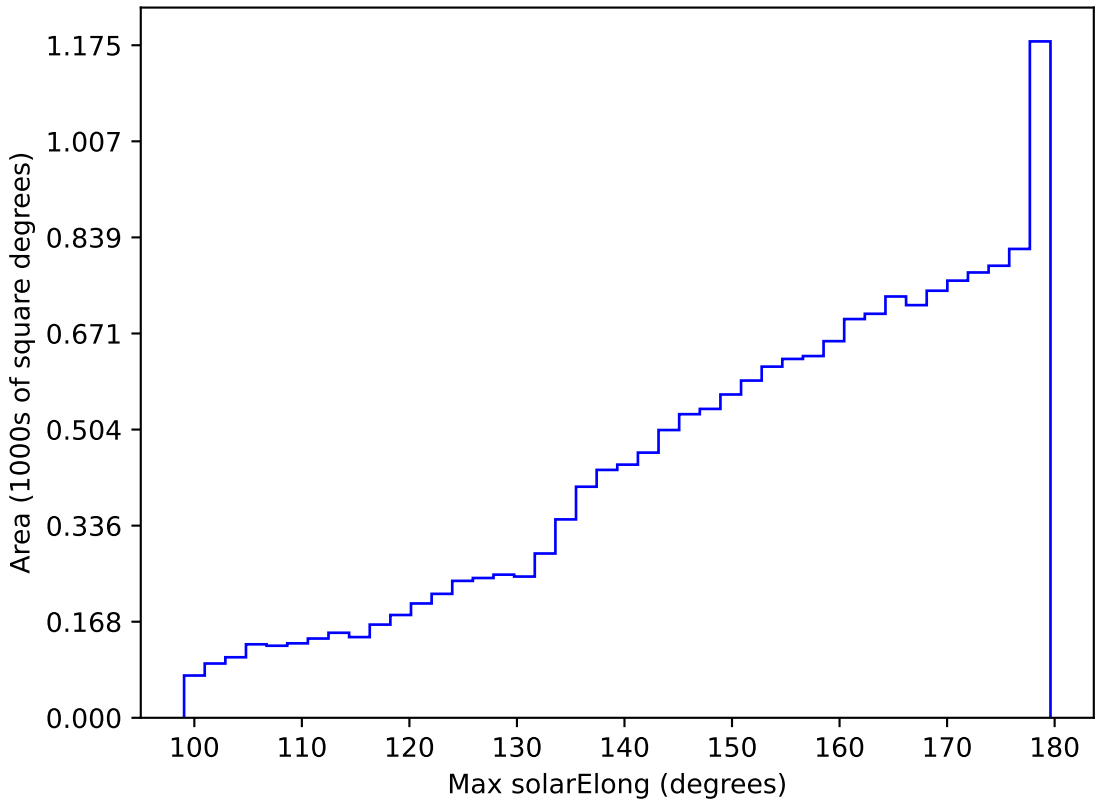
too_elab_r8_d3_giz_v3.4_10yrs WFD all bands: Max solarElong
