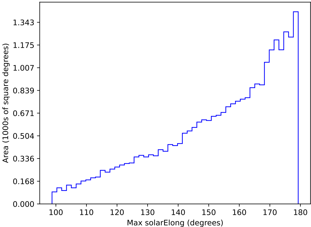
too_elab_r8_d3_giz_v3.4_10yrs All sky z band: Max solarElong
