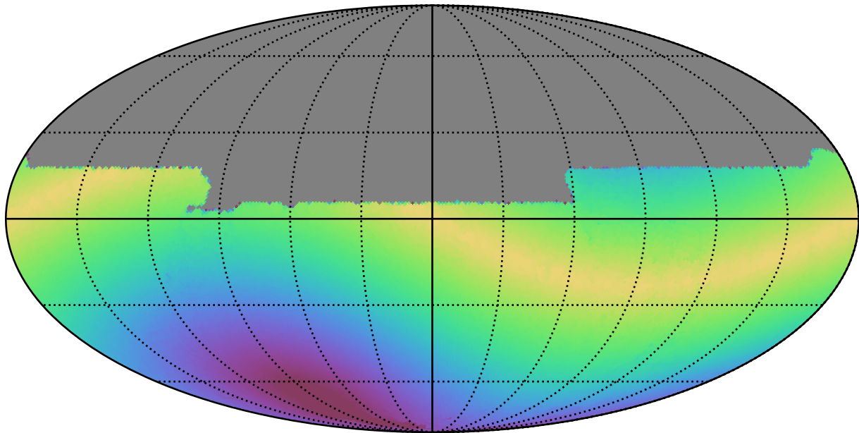
too_elab_r8_d3_giz_v3.4_10yrs All sky y band: Max solarElong
