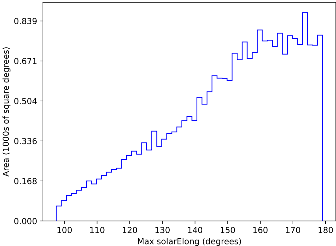
too_elab_r8_d3_giz_v3.4_10yrs All sky u band: Max solarElong
