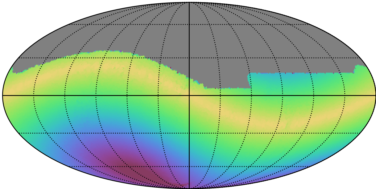
too_elab_r8_d3_giz_v3.4_10yrs All sky r band: Max solarElong
