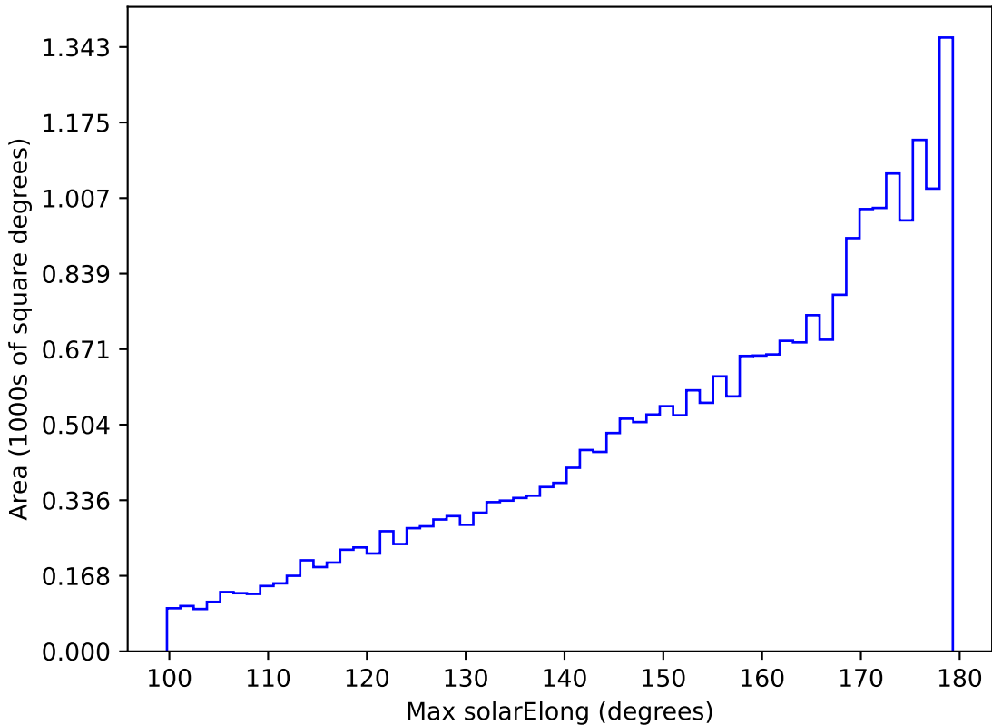
too_elab_r8_d3_giz_v3.4_10yrs All sky r band: Max solarElong
