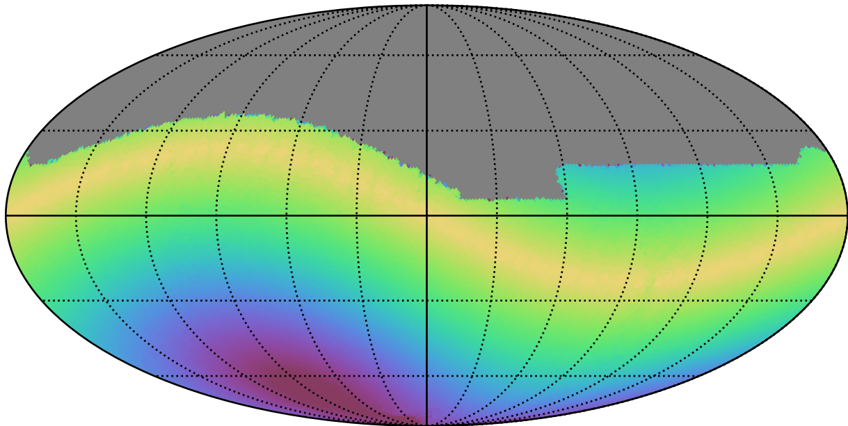
too_elab_r8_d3_giz_v3.4_10yrs All sky i band: Max solarElong
