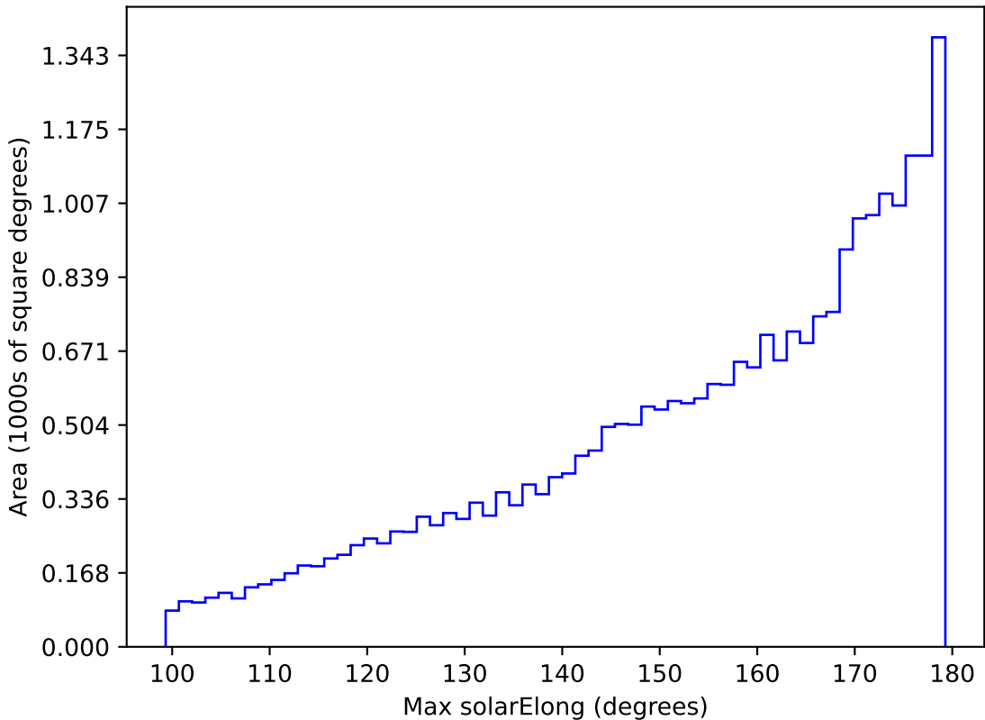
too_elab_r8_d3_giz_v3.4_10yrs All sky i band: Max solarElong
