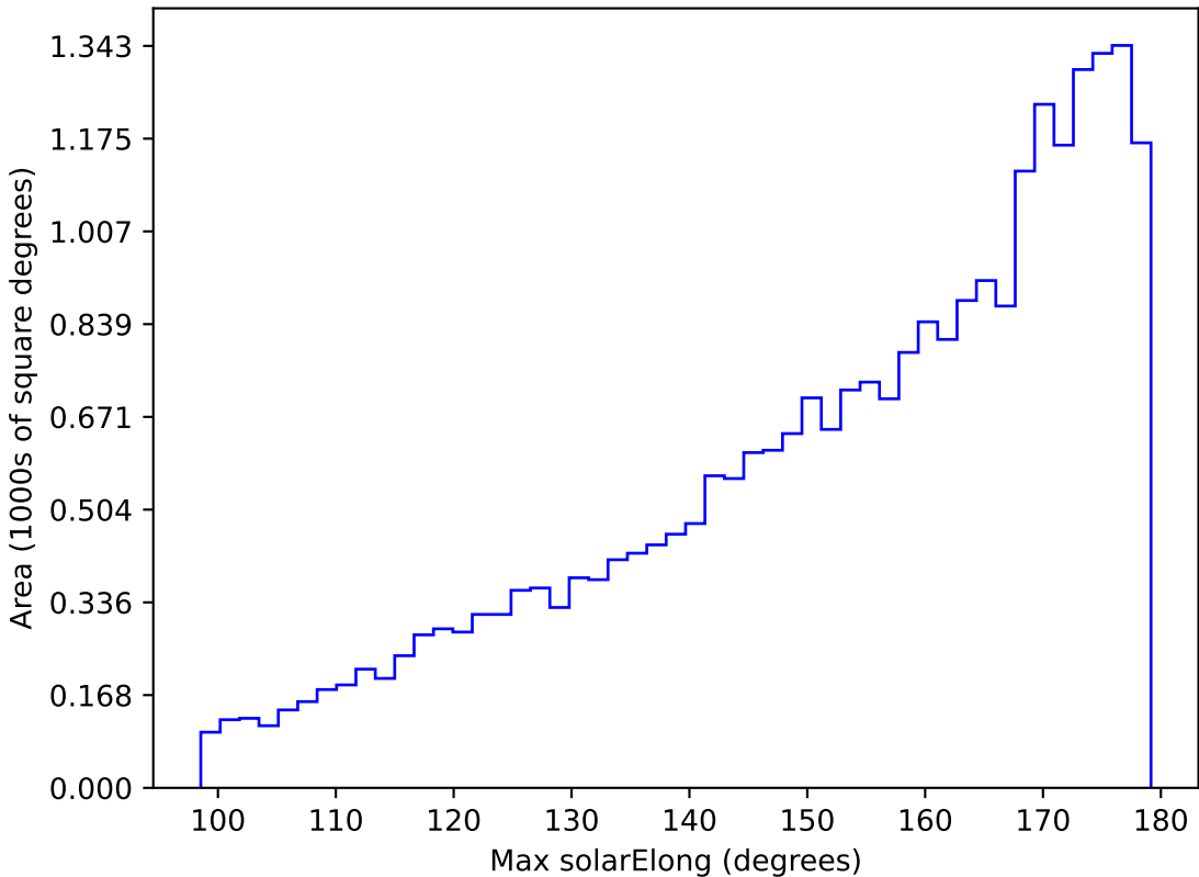
too_elab_r8_d3_giz_v3.4_10yrs All sky g band: Max solarElong
