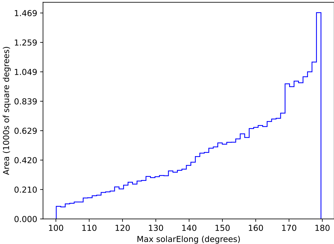
too_elab_r8_d3_giz_v3.4_10yrs All sky all bands: Max solarElong
