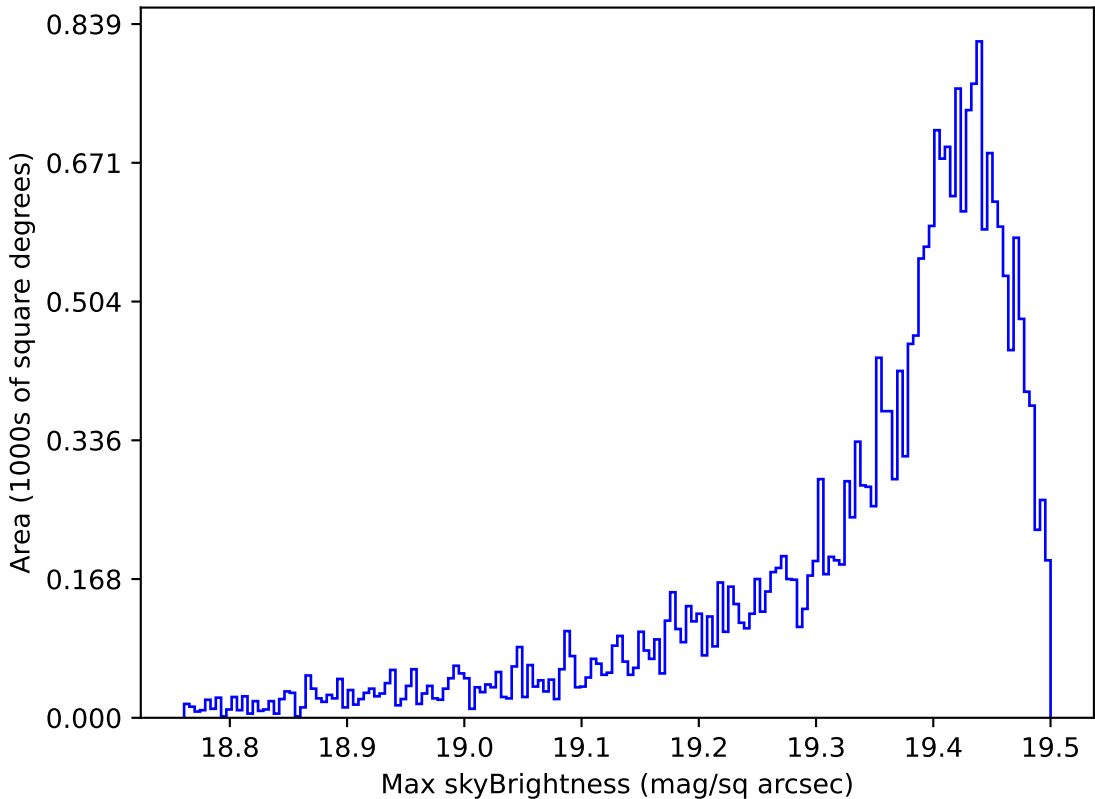
too_elab_r8_d3_giz_v3.4_10yrs Yr 1 z band: Max skyBrightness
