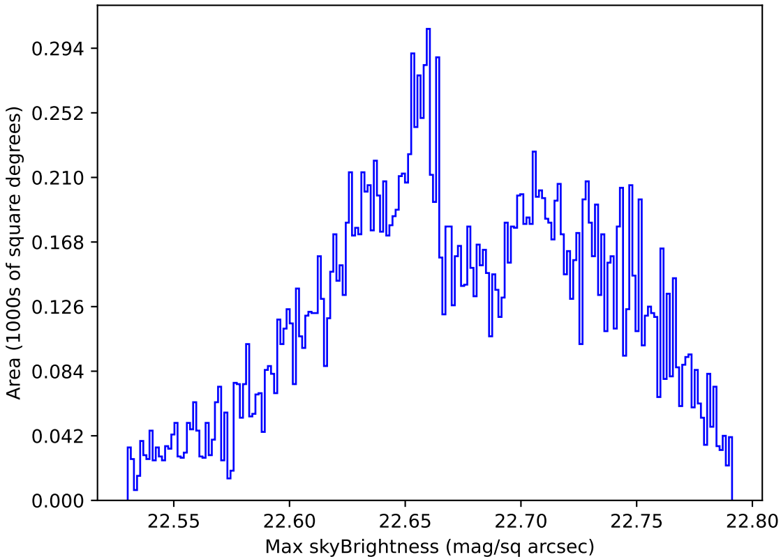
too_elab_r8_d3_giz_v3.4_10yrs Yr 1 u band: Max skyBrightness
