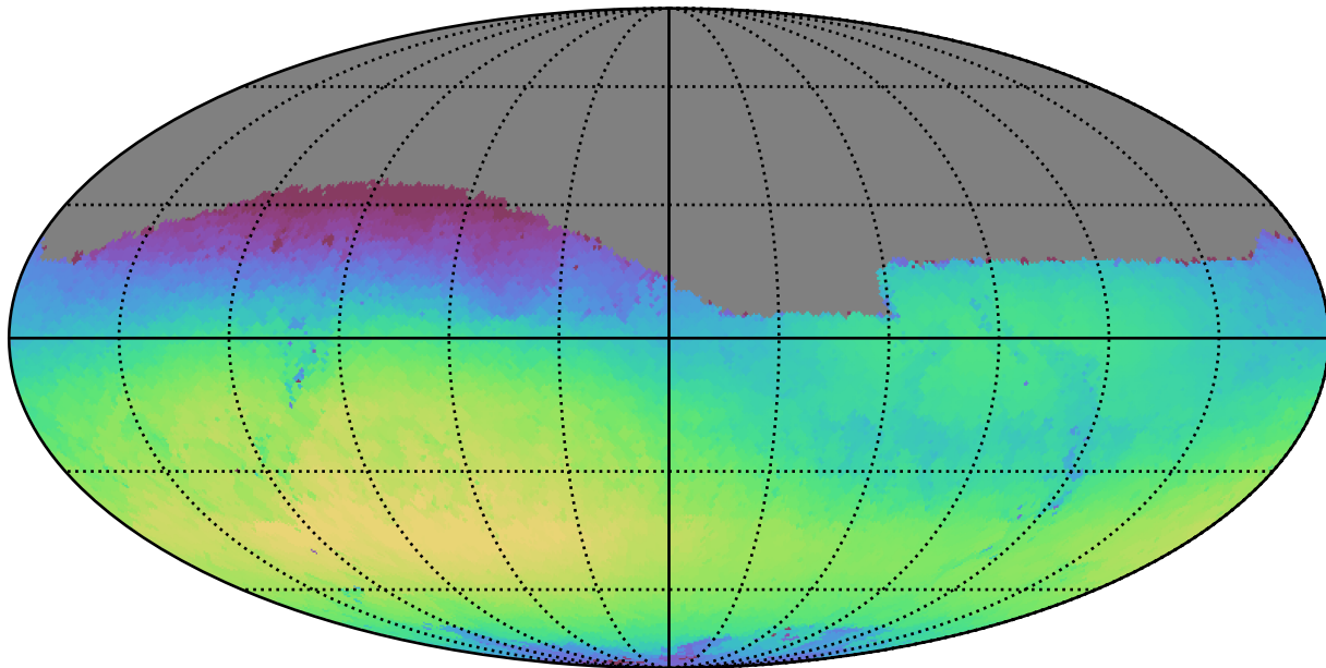
too_elab_r8_d3_giz_v3.4_10yrs Yr 1 r band: Max skyBrightness
