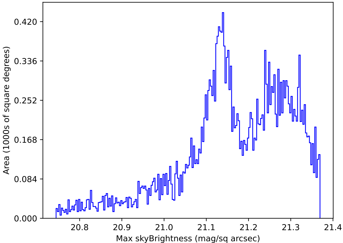
too_elab_r8_d3_giz_v3.4_10yrs Yr 1 r band: Max skyBrightness
