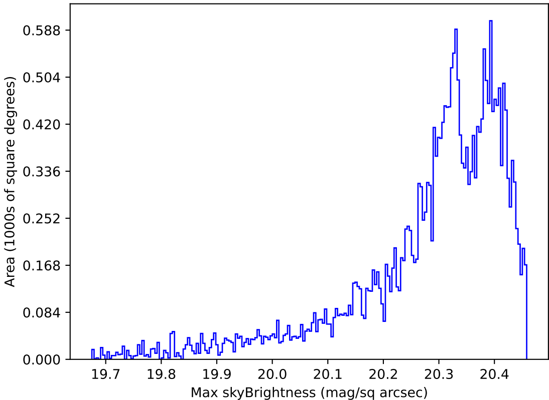
too_elab_r8_d3_giz_v3.4_10yrs Yr 1 i band: Max skyBrightness
