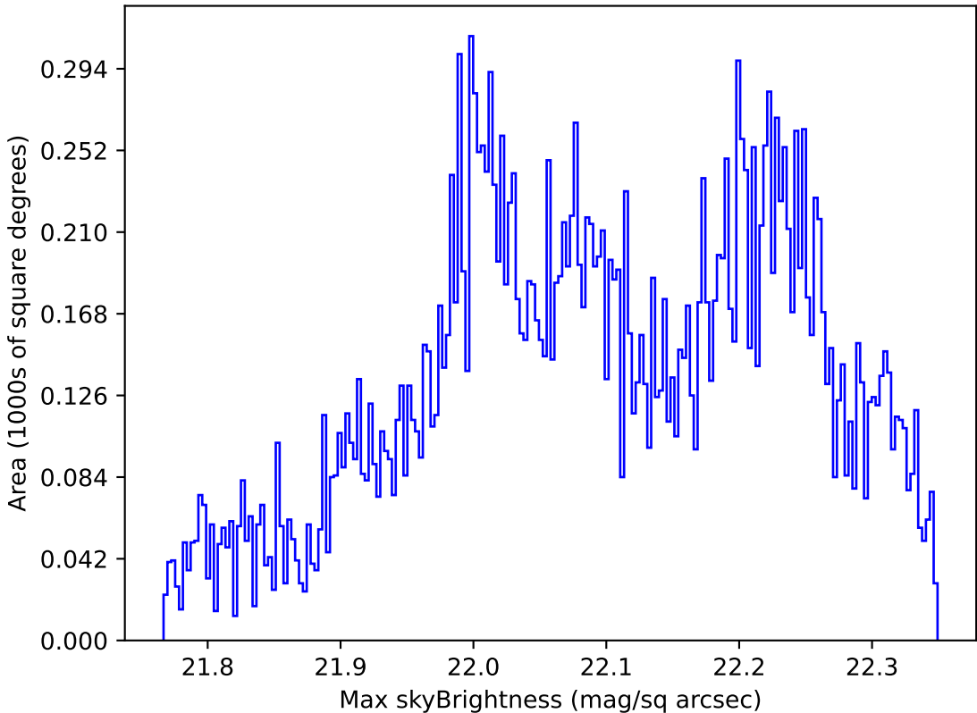
too_elab_r8_d3_giz_v3.4_10yrs Yr 1 g band: Max skyBrightness
