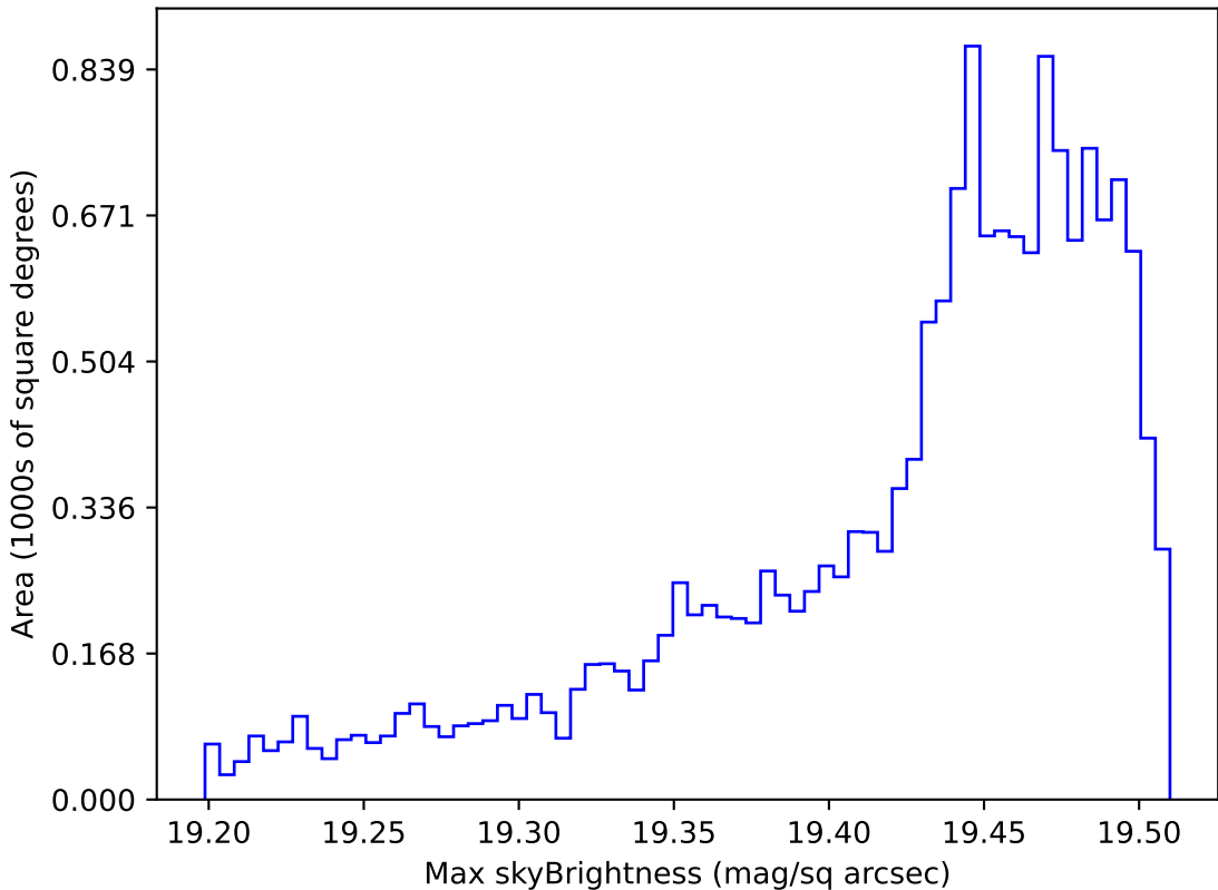
too_elab_r8_d3_giz_v3.4_10yrs WFD z band: Max skyBrightness
