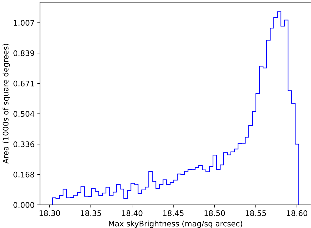
too_elab_r8_d3_giz_v3.4_10yrs WFD y band: Max skyBrightness
