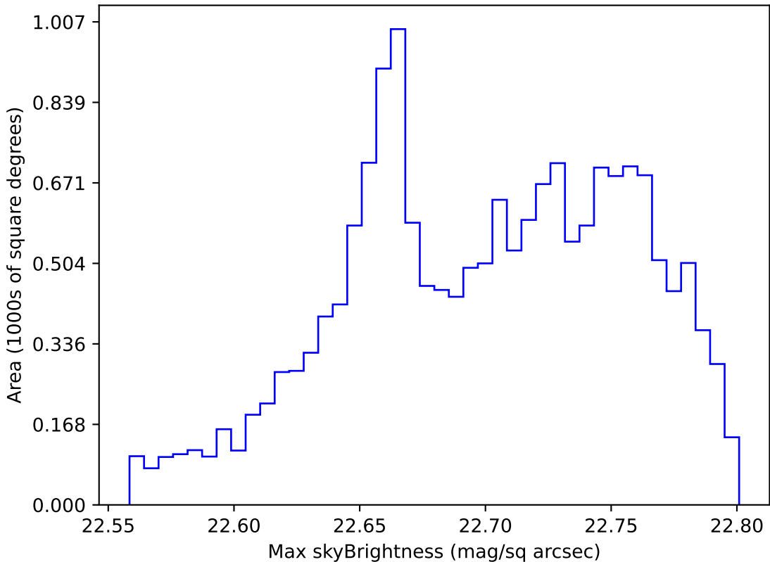
too_elab_r8_d3_giz_v3.4_10yrs WFD u band: Max skyBrightness
