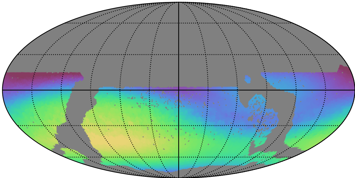
too_elab_r8_d3_giz_v3.4_10yrs WFD r band: Max skyBrightness
