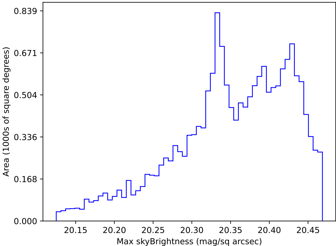
too_elab_r8_d3_giz_v3.4_10yrs WFD i band: Max skyBrightness
