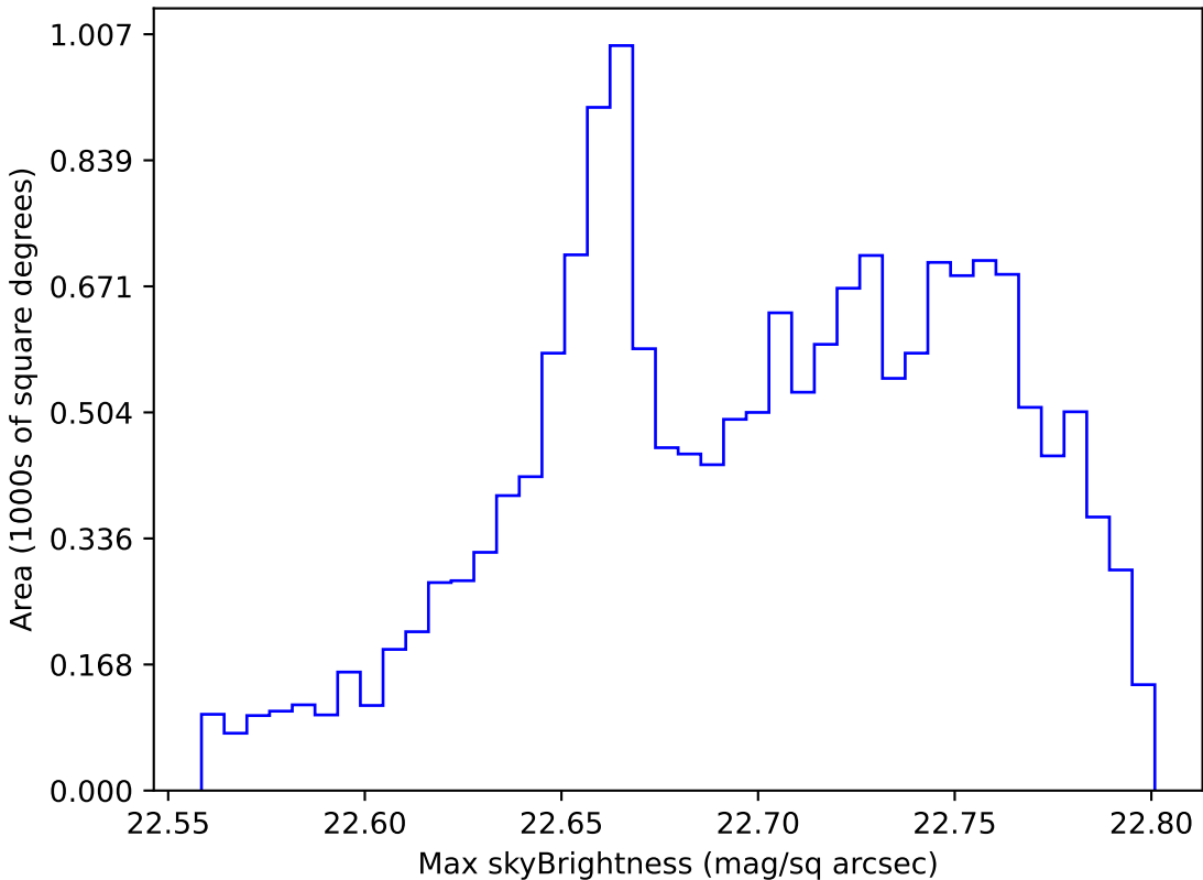
too_elab_r8_d3_giz_v3.4_10yrs WFD all bands: Max skyBrightness
