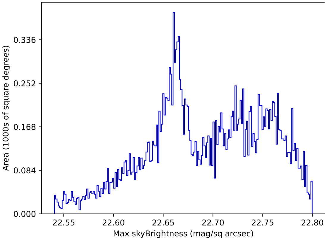
too_elab_r8_d3_giz_v3.4_10yrs All sky u band: Max skyBrightness
