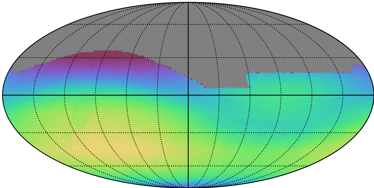
too_elab_r8_d3_giz_v3.4_10yrs All sky r band: Max skyBrightness
