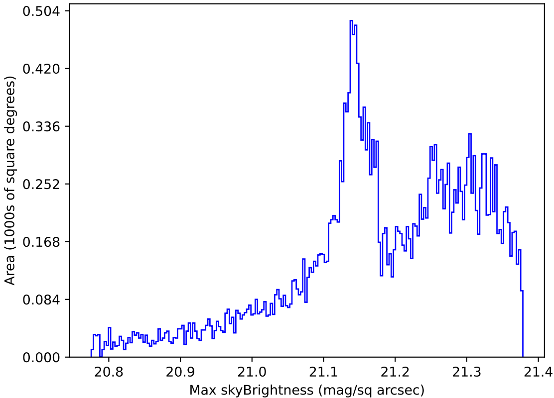
too_elab_r8_d3_giz_v3.4_10yrs All sky r band: Max skyBrightness
